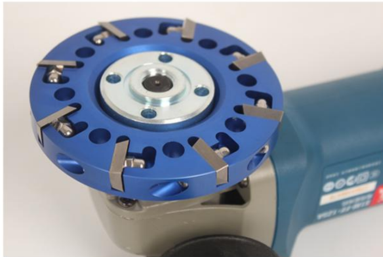
Hoof Trimming Machine with 8 cutter
